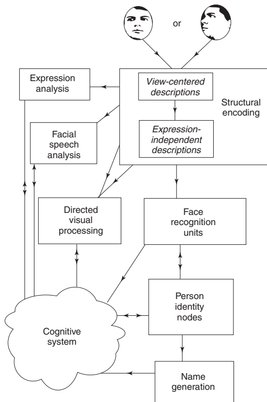
Cognition Model.
