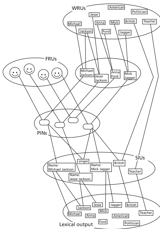
PDP Model.
