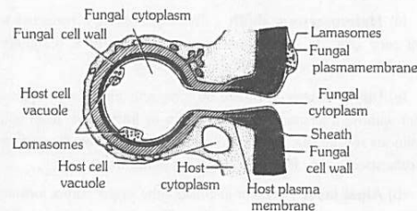
Fig : 1.4-3 Albugo – Ultra structure of haustorium (diagrammatic)
