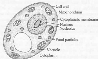
Fig : 1.4-2 Electron micrograph of single yeast cell
