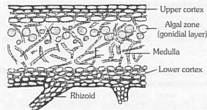
Fig : 1.4-4 Transverse section of a foliose lichen
