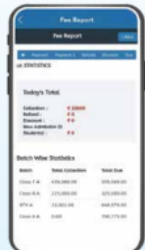
FEE REPORT
