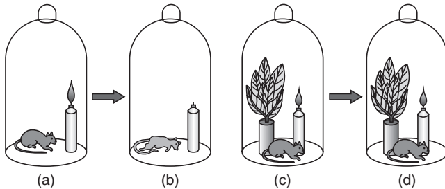
Priestley's experiment
