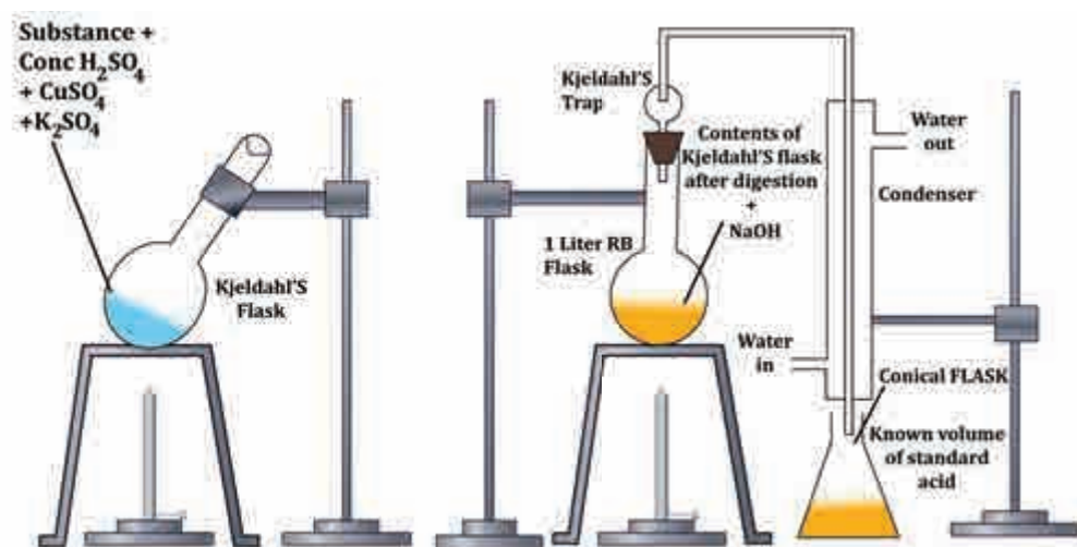
Fig 11.3 Kjeldahl's method
