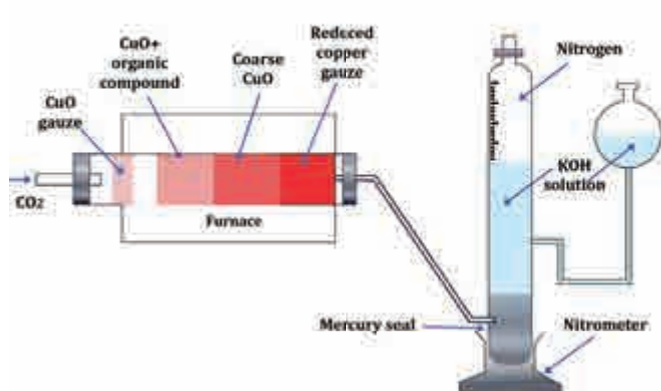
Fig 11.4 Dumas Method
