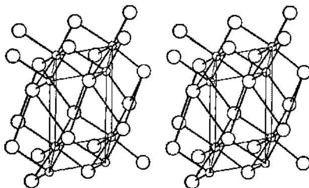
Fig. 7.8 Stereoview of the unit cell of the cadmium iodide, \text{CdI}_2 , structure type; hexagonal, space group P\bar{3}m1 . Large circles, I; small circles, Cd. [From Ladd, M. F. C. Structure and Bonding in Solid State Chemistry ; Ellis Horwood: Chichester, 1979. Reproduced with permission.]
