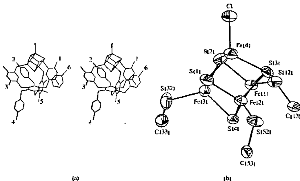
Fig. 19.14 Model compound for a cubane-type Fe_4 cluster with a trithiol ligand. (a) Stereoview of [Fe_4S_4(\text{trithiol})L'] ; (b) close-up view of the Fe-S cluster. [From Stack, T. D. P.; Holm, R. H. J. Am. Chem. Soc. 1988, 110, 2484–2494. Reproduced with permission.]
