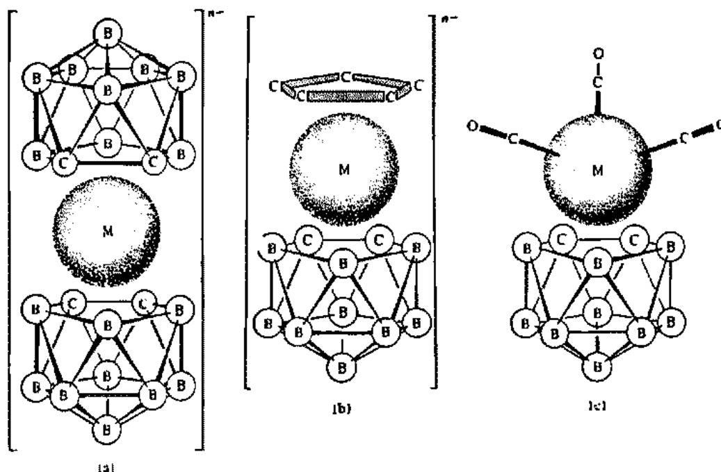
Fig. 16.53 Structures of some carbolly metallocene compounds. (a) Dicarbolyl species: M = \text{Fe} , n = 2 , and M = \text{Co} , n = 1 are isoelectronic with ferrocene and cobaltocenium ion; M = \text{Fe} , n = 1 is isoelectronic with ferrocenium ion; (b) mixed carbolly-cyclopentadienyl analogue of ferrocene, n = 1 ; (c) mixed carbolly-carbonyl compound, M = \text{Mn} , R^2 . [(a) and (b) from Hawthorne, M. F.; Andrews, T. D. J. Am. Chem. Soc. 1965, 87, 2496; (c) from Adler, R. G.; Hawthorne, M. F. J. Am. Chem. Soc. 1970, 92, 6174. Reproduced with permission.]
