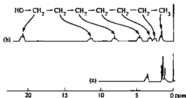
Fig. 14.13 Proton NMR spectra (60 MHz) of 1-heptanol. (a) Spectrum of 0.3 M 1-heptanol in \text{CDCl}_3 . (b) Spectrum of 0.78 molar ratio of tris-(dipivaloyl-methanato)-europium(III)/1-heptanol in \text{CDCl}_3 . [From Rabenstein, D. L. Anal. Chem. 1971, 43, 1599-1605, as modified by Mayo, B. C. Chem. Soc. Rev. 1973, 2, 49-74. Reproduced with permission.]
