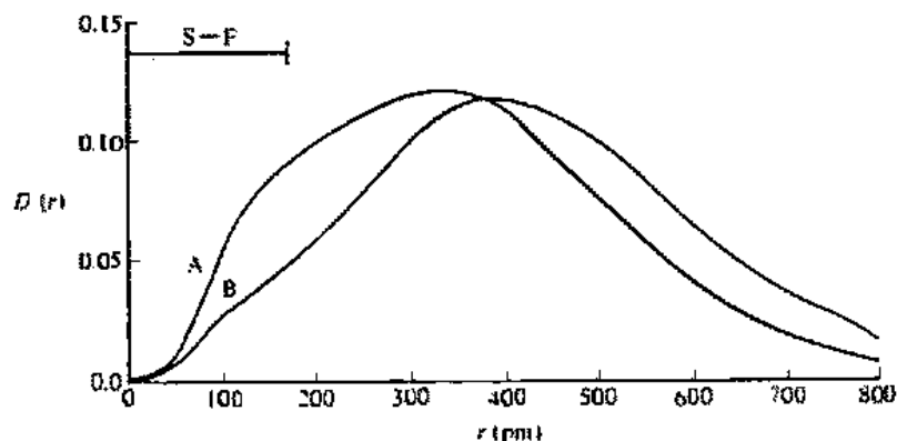
Fig. 18.3 The 3 d orbital distribution functions in d 1 configurations (A) in the 4 D term of P ( s 1 p 3 d 1 ); (B) in the 2 D term of S ( s 2 p 3 d 1 ). Line represents a typical S—F bond length. [Modified from Mitchell, K. A. R. Chem. Rev. 1969, 69, 157. Reproduced with permission.]
