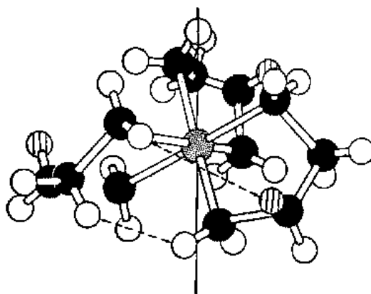
Fig. 12.30 The nb conformer of the \Delta or \Lambda isomer of tris(diamine)metal complexes. The hatched circles represent the positions of the methyl groups in the propylenediamine complex. For propylenediamine this represents the \Delta\delta\delta\delta or \Lambda\delta\delta\delta isomer. (Modified from Corey, E. J.; Bailar, J. C., Jr. J. Am. Chem. Soc. 1959, 81, 2620-2629. Reproduced with permission.)
