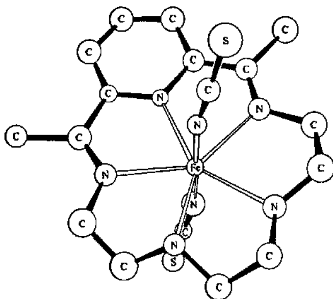
Fig. 12.32 Molecular structure of the seven-coordinate complex of iron involving 2,13-dimethyl-3,6,9,12,18-pentazaabicyclo-[12.3.1]-octadeca-1(18),2,12,14,16-pentaene and two axial \text{SCN}^- ligands. Hydrogen atoms omitted. [From Fleischer, E.; Hawkinson, S. J. Am. Chem. Soc. 1967, 89, 720-721. Reproduced with permission.]
