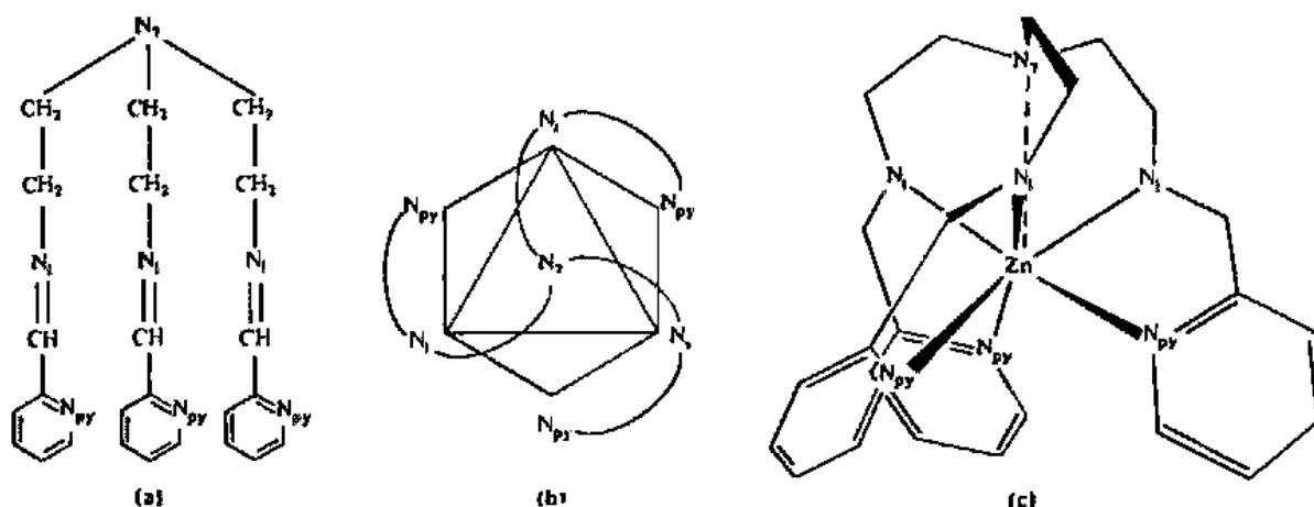
Fig. 12.35 [M(\text{py}_3\text{tren})]^{3+} complexes: (a) The \text{py}_3\text{tren} ligand: \text{N}(\text{CH}_2\text{CH}_2\text{N}=\text{CHC}_5\text{H}_4\text{N})_3 ; the nitrogen atoms are labeled \text{N}_{\text{py}} , the pyridine nitrogen, \text{N}_i , the imine nitrogen, and \text{N}_7 , the seventh or unique nitrogen atom; (b) a diagrammatic representation of the [M(\text{py}_3\text{tren})]^{3+} complex, viewed down the threefold axis; (c) the molecular structure of the zinc(II) complex, viewed perpendicular to the threefold axis. [Courtesy of E. C. Lingafelter.]
