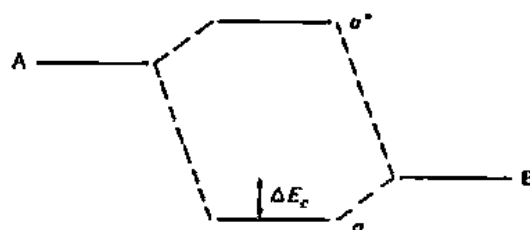
Fig. 5.22 Heteronuclear molecule, A^{5+}B^{5-} , with relatively small electronegativity difference between A and B. Covalency reduced with respect to A_2 (Fig. 5.21), but still more important than the ionic contribution.
