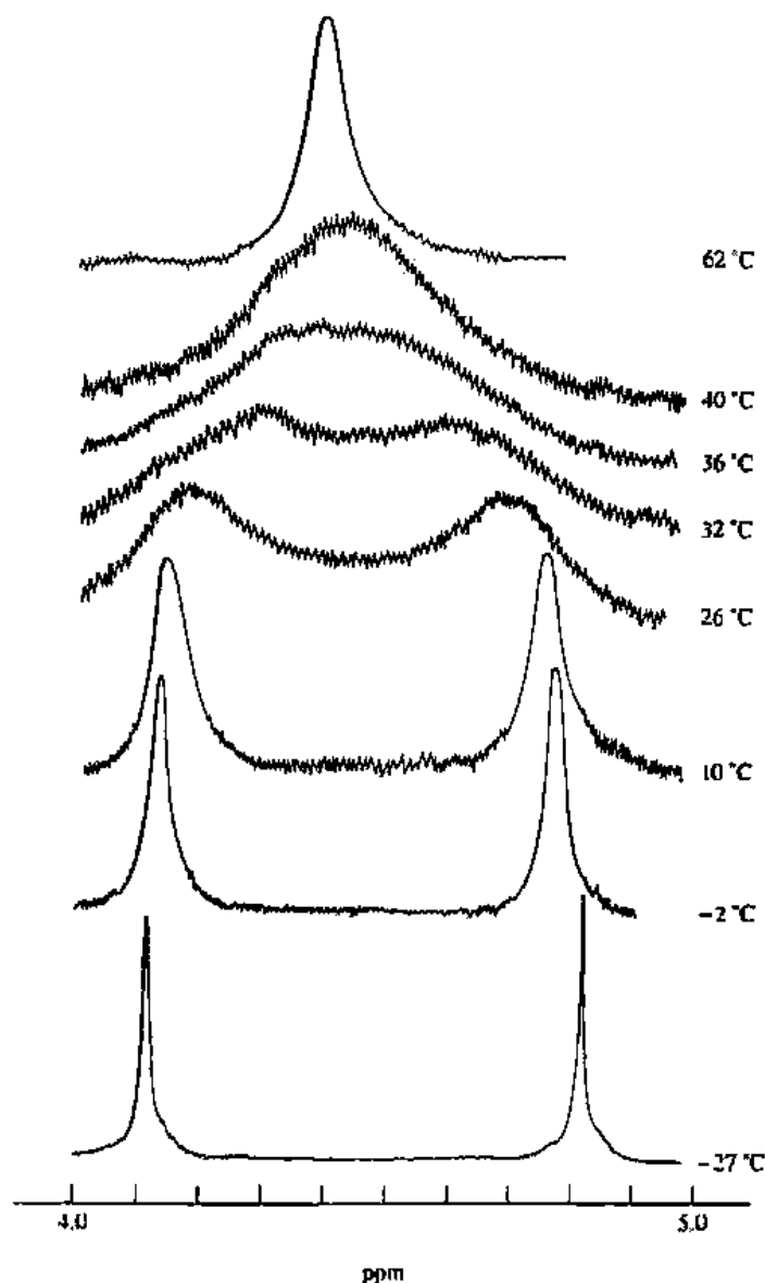
Fig. 15.52 Proton NMR spectra of (\eta^1\text{-C}_5\text{H}_5)(\eta^5\text{-C}_5\text{H}_5)_2\text{Ti} from -27 to +62 °C. The separate resonances observed at low temperature for the two types of Cp rings gradually broaden and collapse, giving a single line at 62 °C. [From Cotton, F. A. In Dynamic Nuclear Magnetic Resonance Spectroscopy ; Jackman, L. M., Cotton, F. A., Eds.; Academic: New York, 1975; Chapter 10. Used with permission.]
