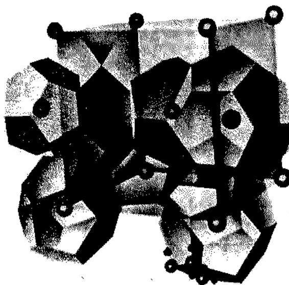
Fig. 17.1 The structure of the xenon hydrate clathrate. The xenon atoms occupy the centers of regular pentagonal dodecahedra of water molecules (cf. Fig. 8.8).
