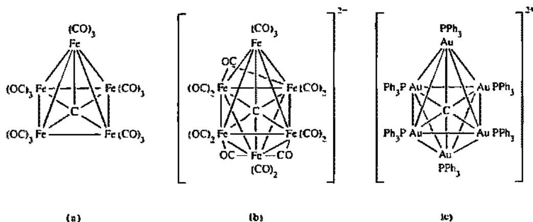
Fig. 15.21 Structural examples of carbido complexes: (a) \text{Fe}_5(\text{CO})_{15}\text{C} , (b) [\text{Fe}_6(\text{CO})_{16}\text{C}]^{2-} , and (c) [\text{Au}_6(\text{PPh}_3)_6\text{C}]^{2+} . [From Bray, E. H.; Dahl, L. F.; Hübel, W.; Wampler, D. L. J. Am. Chem. Soc. 1962, 84, 4633–4639 (a); Bradley, J. S. Adv. Organomet. Chem. 1983, 22, 1–58 (b); Scherbaum, F.; Grohmann, A.; Huber, B.; Kruger, C.; Schmidbaur, H. Angew. Chem. Int. Ed. Engl. 1988, 27, 1544–1546 (c). Used with permission.]
