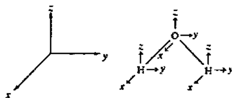
Fig. 3.22 Cartesian displacement vectors for the water molecule.
