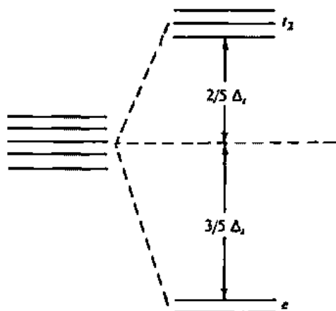
Fig. 11.11 Splitting of d orbitals in a tetrahedral field.
