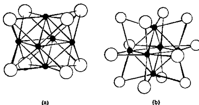
Fig. 16.64 The structure of the \text{Mo}_6\text{Cl}_8^{4+} ion; ● = Mo, ○ = Cl. (b) The structure of the \text{M}_6\text{X}_{12}^{2+} ions; ● = Nb, Ta; ○ = Cl, Br. [From Cotton, F. A. Acc. Chem. Res. 1969, 2, 240. Reproduced with permission.]
