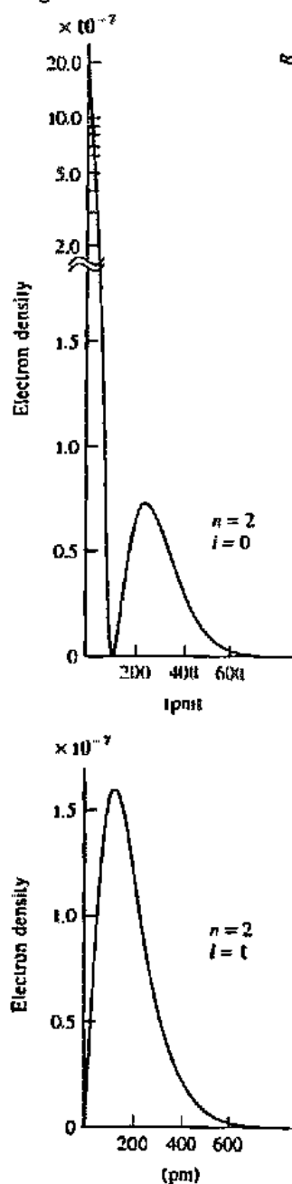
Fig. 2.2 Radial density functions for n = 2 for the hydrogen atom. These functions give the relative electron density ( e \text{ pm}^{-3} ) as a function of distance from the nucleus. They were prepared by squaring the wave functions given in Fig. 2.1.
