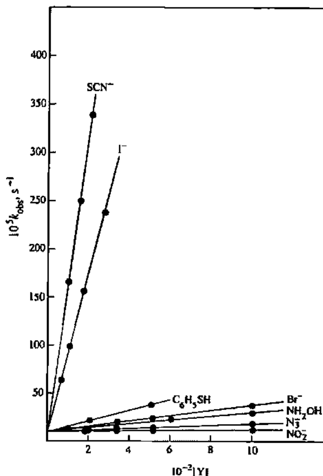
Fig. 13.1 Rate constants ( k_{\text{obs}}, \text{s}^{-1} ) as a function of nucleophile concentration ( [Y] ) for reaction of \text{trans-}[\text{Pt}(\text{Py})_2\text{Cl}_2] with various nucleophiles in methanol at 30^\circ\text{C} . [From Belluco, U.; Cattalini, L.; Basolo, F.; Pearson, R. G.; Turco, A. J. Am. Chem. Soc. 1965, 87, 241-246. Used with permission.]
