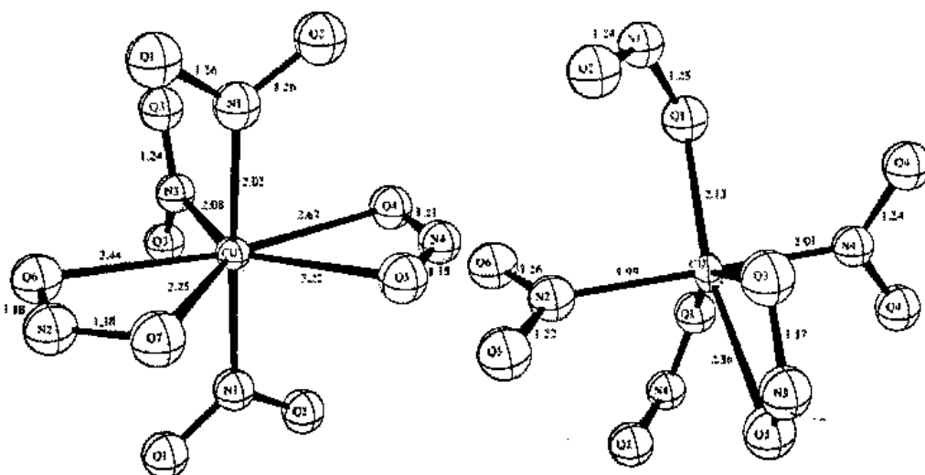
Fig. 12.52 Two forms of the [\text{Cu}(\text{NO}_2)_5]^{3-} ion. All bond distances in angstroms. [From Klenderman, K. A.; Hamilton, W. C.; Eernal, I. Inorg. Chem. Acta 1977, 23, 117-129. Reproduced with permission.]
