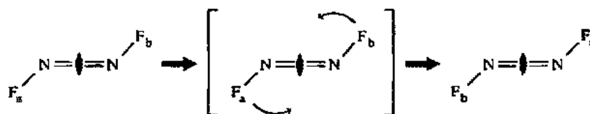
Fig. 3.5 The two-fold rotational axis in trans -dinitrogen difluoride. The two-fold axis is perpendicular to the plane of the paper and denoted by the symbol \perp .
