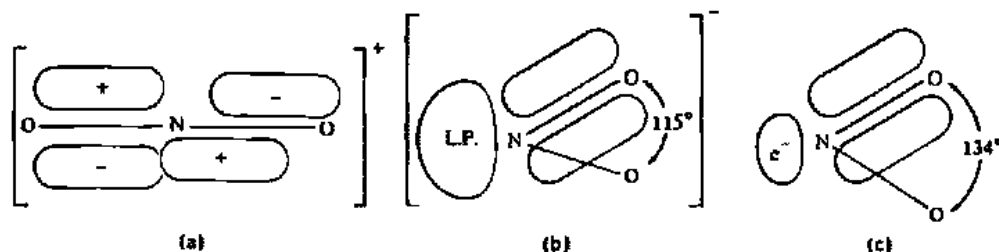
Fig. 6.8 (a) The linear nitryl ion, \text{NO}_2^+ . (b) The effect of the lone pair in the nitrite ion, \text{NO}_2^- . Resonance has been omitted to simplify the discussion. (c) The effect of the unpaired electron, half of a lone pair, in nitrogen dioxide.
