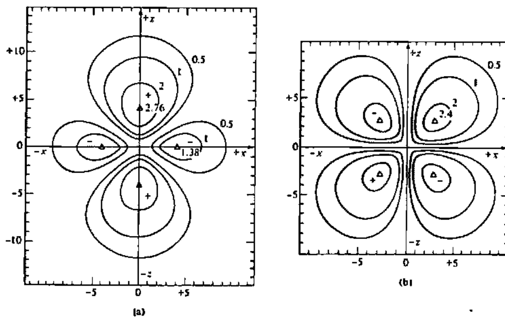
Fig. 11.4 Electron density contours for (a) d_{x^2-y^2} and (b) d_{xz} orbitals. The triangles represent points of maximum electron density. [From Perlmuter-Hayman, B. J. Chem. Educ. 1969, 46, 428-430. Reproduced with permission.]
