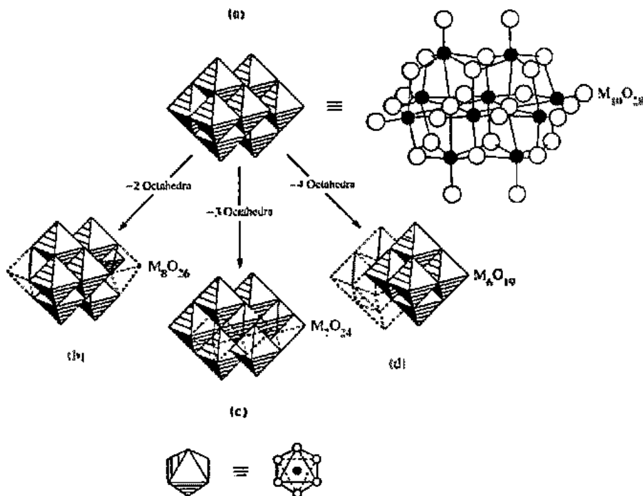
Fig. 16.10 The structures of edge-shared isopoly anions showing their relation to the M_{10}O_{28} structure: (a) M = V ; (b) M = Mo ; (c) M = Mo ; (d) M = Nb, Ta . [From Kepert, D. L., Inorg. Chem. 1969, 8, 1556, and Day, V. W.; Klemperer, W. G.; Maltbie, D. J. J. Am. Chem. Soc. 1987, 109, 2991–3002. Reproduced with permission.]
