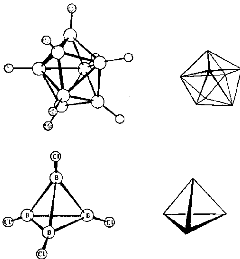
Fig. 16.48 (a) The structure of the [\text{B}_n\text{H}_n]^{2-} anion compared to an idealized dodecahedron. [From Guggenberger, L. J. Inorg. Chem. 1969, 8, 2771. Reproduced with permission.] (b) Molecular structure of \text{B}_3\text{Cl}_4 compared to an idealized tetrahedron. [From Muetterties, E. L. The Chemistry of Boron and Its Compounds ; Wiley: New York, 1967. Reproduced with permission.]
