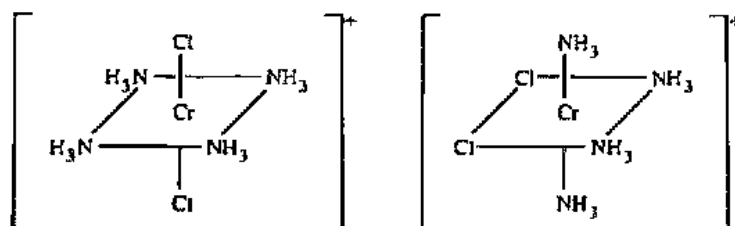
1. trans -isomer
