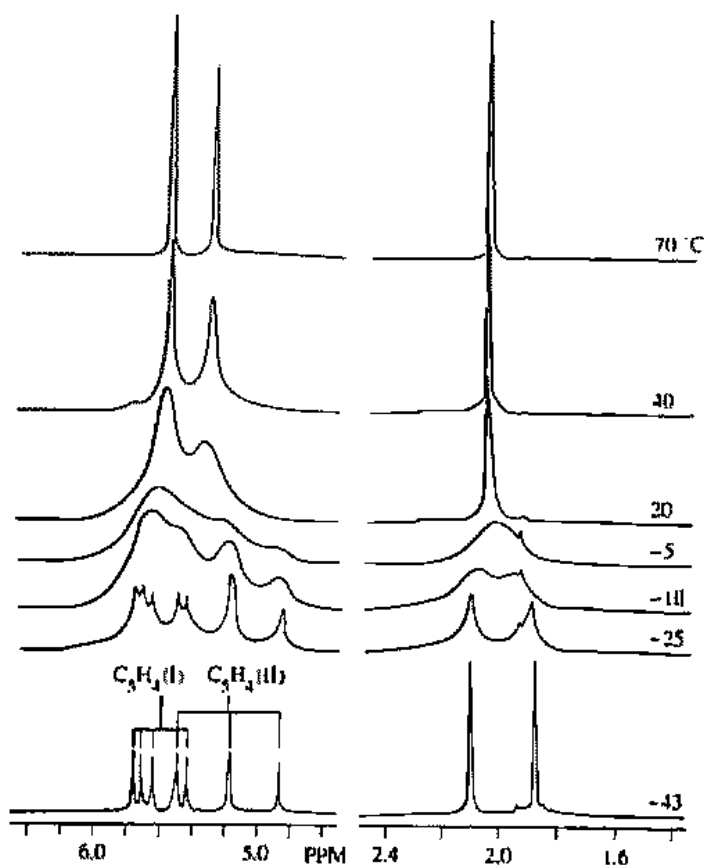
Fig. 15.57 Variable temperature 500 MHz proton NMR spectra of [(\text{MeC}_3\text{H}_4)_4\text{Ru}_4\text{S}_4]^{2+} in the \text{CH}_3 and \text{C}_3\text{H}_3 regions. The spectra provide evidence for a metal-metal bond migration having an activation energy of 52 \text{ kJ mol}^{-1} . [From Houser, E. J.; Amarasekera, J.; Rauchfuss, T. B.; Wilson, S. R. J. Am. Chem. Soc. 1991, 113, 7440-7442. Reproduced with permission.]
