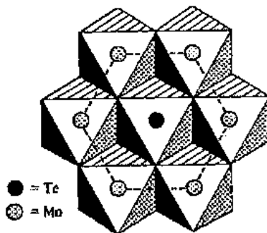
Fig. 16.15 The structure of the 6-molybdotellurate anion, [\text{TeMo}_6\text{O}_{24}]^{6-} [Adapted, in part, from Kepert, D. L. Prog. Inorg. Chem. 1965, 4, 199. Reproduced with permission.]
