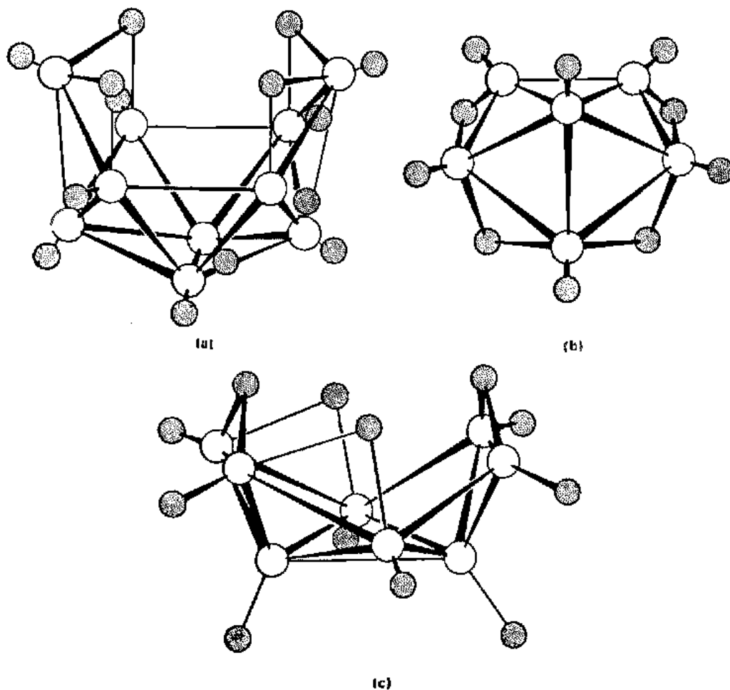
Fig. 16.47 Molecular structures of boranes related to [\text{B}_{12}\text{H}_{12}]^{2-} : (a) decaborane(14) formed by removal of atoms B 1 and B 6 ; (b) hexaborane(10). Note that the pentagonal pyramid is an apical fragment of an icosahedron. (c) Octaborane(12) related to [\text{B}_{12}\text{H}_{12}]^{2-} by removal of B 1 , B 2 , B 5 , B 6 . [From Muettieries, E. L. The Chemistry of Boron and Its Compounds ; Wiley: New York, 1967. Reproduced with permission.]
