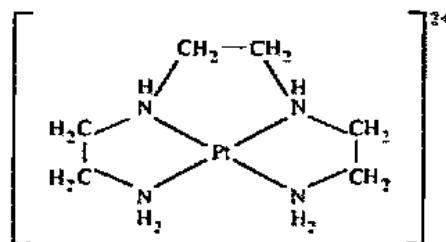
4. tetradentate chelation
