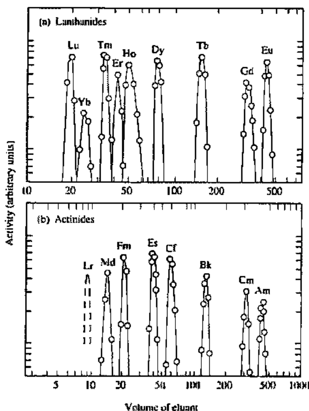
Fig. 14.11 Elution of trivalent lanthanide and actinide ions on a Dowex 50 cation-exchange resin with an ammonium \alpha -hydroxyisobutyrate eluant. The band for Lr^{3+} is predicted. [From Katz, J. J.; Morss, L. R.; Seaborg, G. T. In The Chemistry of the Actinide Elements ; Katz, J. J.; Morss, L. R.; Seaborg, G. T., Eds.; Chapman and Hall: New York, 1986; Vol. 2, pp 1131-1133. Reproduced with permission.]
