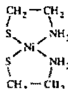
6. cis -isomer
