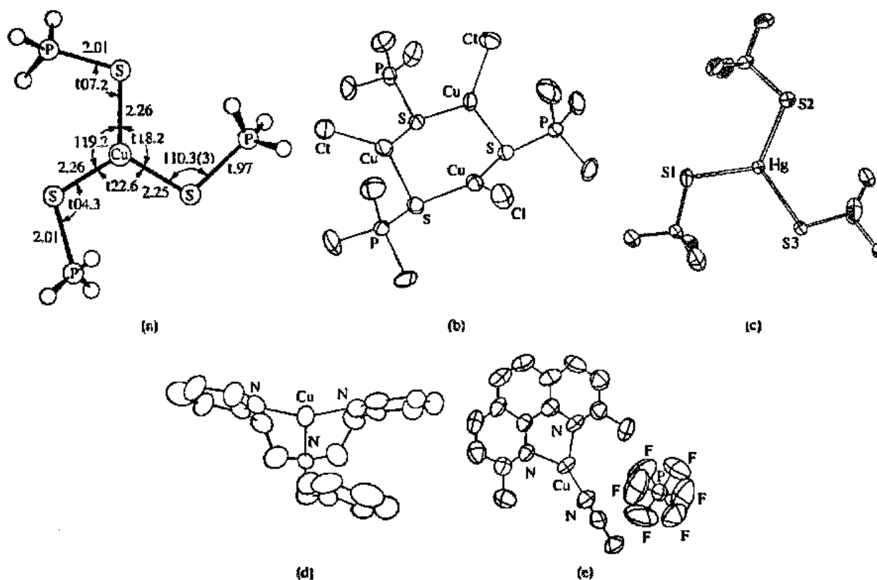
Fig. 12.1 Three-coordinate complexes: (a) \text{Cu}[\text{SP}(\text{Me})_3]^+ ; (b) [\text{Cu}(\text{SP}(\text{CH}_3)_3)\text{Cl}]_2 ; (c) [\text{Hg}(\text{SBu})_3]^- ; (d) [\text{C}_6\text{H}_5\text{CH}_2\text{N}(\text{CH}_2\text{CH}_2\text{C}_5\text{H}_4\text{N})_2\text{Cu}]^+ ; (e) [(\text{CH}_3\text{CN})\text{CuN}_2\text{C}_{12}\text{H}_8(\text{CH}_3)_2]\text{PF}_6 . Carbon atoms are unmarked and hydrogen atoms have been omitted. [From Eller, P. G.; Corfield, P. W. R. Chem. Commun. 1971, 105–106. Tiethof, J. A.; Stalick, J. K.; Meek, D. W. Inorg. Chem. 1973, 12, 1170–1174. Tiethof, J. A.; Hetey, A. T.; Meek, D. W. Inorg. Chem. 1974, 13, 2505–2509. Watton, S. P.; Wright, J. G.; MacDonnel, F. M.; Bryson, J. W.; Sabat, M.; O'Halloran, T. V. J. Am. Chem. Soc. 1990, 112, 2824–2826. Blackburn, N. J.; Karlin, K. D.; Concannon, M.; Hayes, J. C.; Gultneh, Y.; Zubieta, J. Chem. Commun. 1984, 939–940. Munakata, M.; Maekawa, M.; Kitagawa, S.; Matsuyama, S.; Masuda, H. Inorg. Chem. 1989, 28, 4300–4302. Reproduced with permission.]
