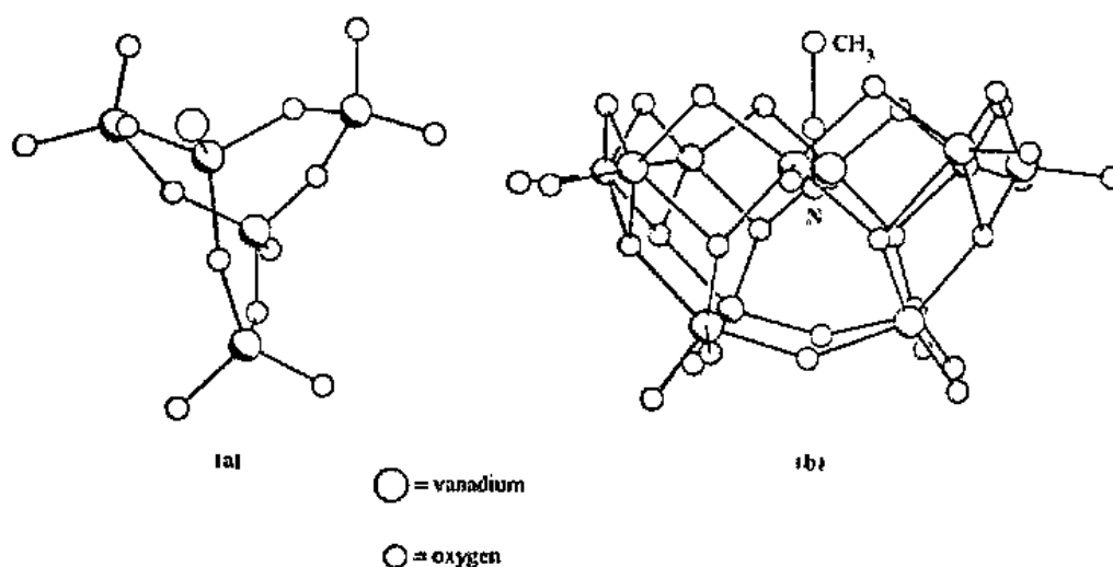
Fig. 16.12 Structures of two oxoanions of vanadium prepared from nonaqueous solvents. (a) [V_3O_{14}]^{3-} . (b) [CH_3CNCV_{12}O_{32}]^{4-} . (The acetonitrile molecule is suspended in the basket denoted by the symbol C.) [From Day, V. W.; Klemperer, W. G.; Yaghi, O. M. J. Am. Chem. Soc. 1989, 111, 4518 and 5959. Reproduced with permission.]
