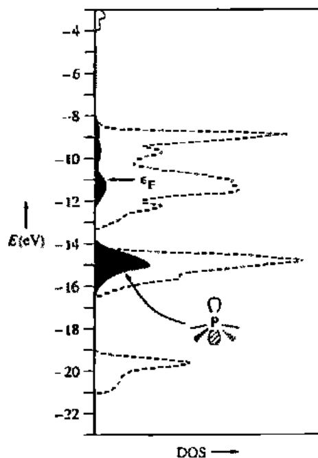
Fig. 7.31 Phosphorus 3p_z orbital contribution (dark area) to the total DOS (dashed line; cf. Figs. 7.29 and 7.30) of the [\text{Mn}_2\text{P}_2]_z^{2-} layer. [Modified from Hoffmann, R.; Zheng, C. J. Phys. Chem. 1985, 89, 4175–4181. Reproduced with permission.]
