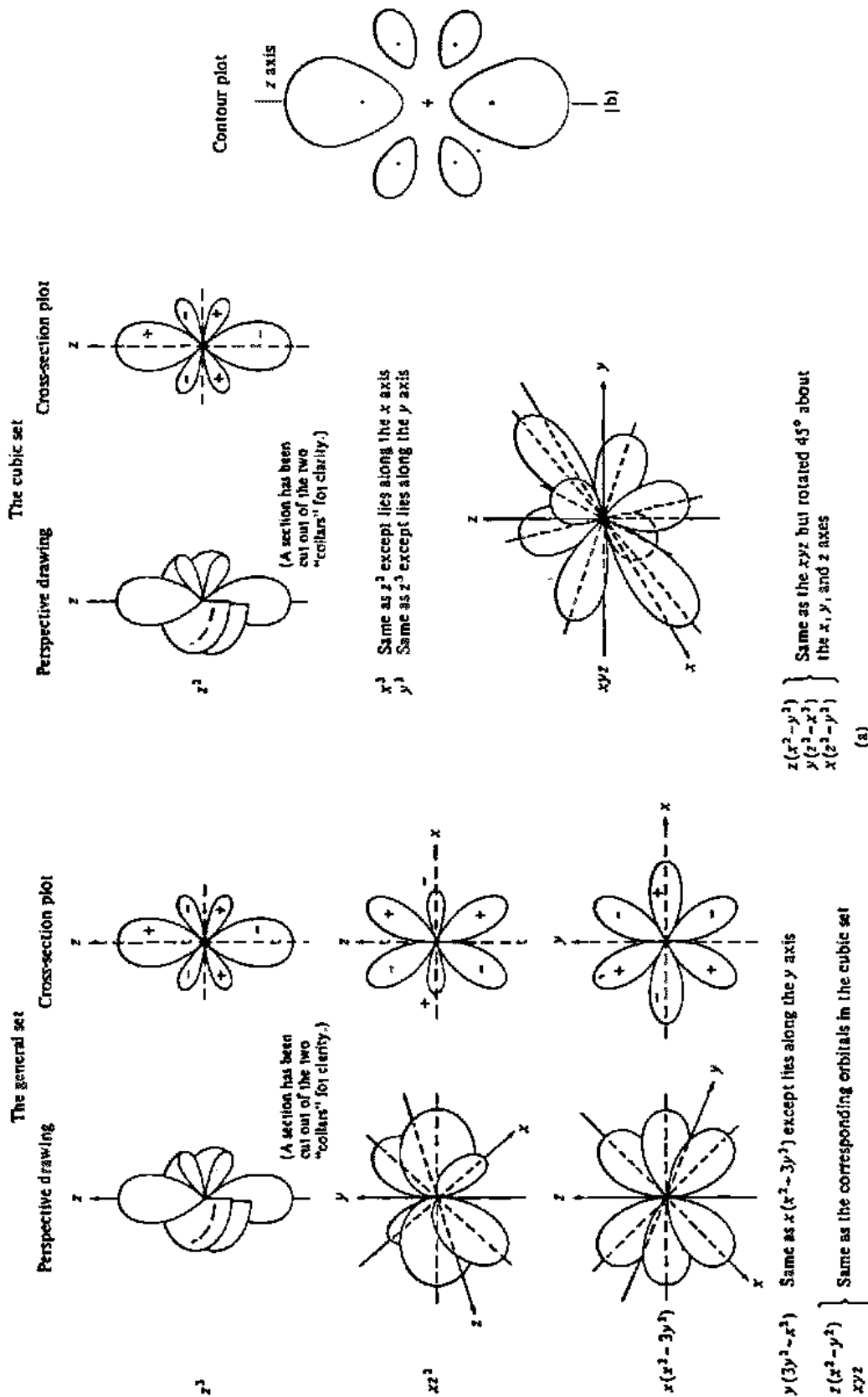
Fig. 14.6 The f orbitals: (a) plots of the angular part of the wave functions of the f orbitals; (b) contours of a 4f orbital. Dots indicate maxima in electron density. The lines are drawn for densities which are 10% of maximum. [(a) From Friedmann, H. G.; Choppin, G. R.; Feuerbacher, D. G. J. Chem. Educ. 1964, 41, 354-358. (b) From Ogrzylo, E. A. J. Chem. Educ. 1965, 42, 150-151. Reproduced with permission.]
