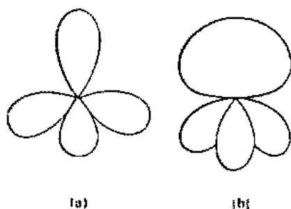
Fig. 6.2 (a) Four equivalent bonding electron pairs. (b) Three bonding electron pairs repelled by a nonbonding pair of electrons.
