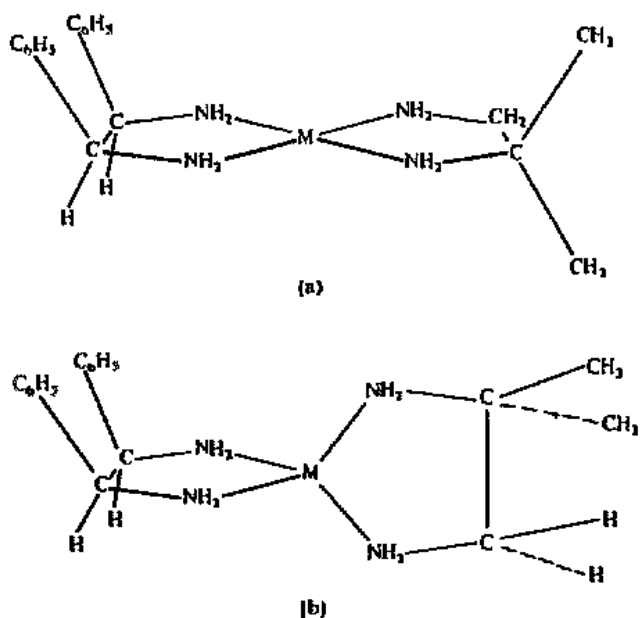
Fig. 12.5 Possible structures of ( meso -stilbenediamine) (isobutylenediamine) palladium(II) and platinum(II) complexes: (a) planar structure, optically active; (b) tetrahedral structure, optically inactive.
