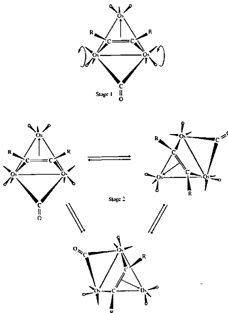
Fig. 15.54 Fluxional behavior of \text{Os}_3(\text{CO})_9(\mu_3\text{-}\eta^2\text{-CH}_3\text{CH}_2\text{C}\equiv\text{CCH}_2\text{CH}_3) . In Stage 1 terminal carbonyl groups are exchanging. In Stage 2 the alkyne ligand moves about the triosmium surface and as it does so, the bridging carbonyl shifts to remain trans to it. [From Rosenberg, E.; Bracker-Novak, J.; Gellert, R. W.; Aime, S.; Gobetto, R.; Osetta, D. J. Organomet. Chem. 1989, 365, 163–185. Reproduced with permission.]
