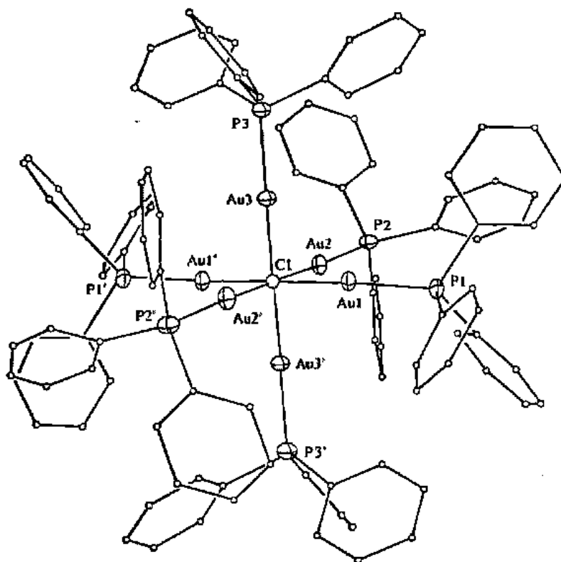
Fig. 18.11 Structure of the "hedgehog" dication, [(\text{Ph}_3\text{PAu})_6\text{Cl}]^{2+} . The inferred Au—Au bonds are not shown. [From Scherbaum, F.; Grohmann, A.; Huber, B.; Krüger, C.; Schmidbaur, H. Angew. Chem. Int. Ed. Engl. 1988, 27, 1544–1546. Reproduced with permission.]
