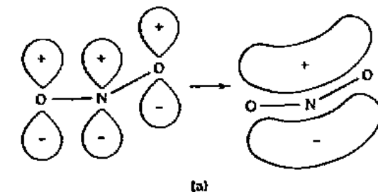
Fig. 5.28 Atomic orbitals (left) and resulting molecular orbitals (right) in the nitrite ion: (a) bonding and (b) antibonding.
