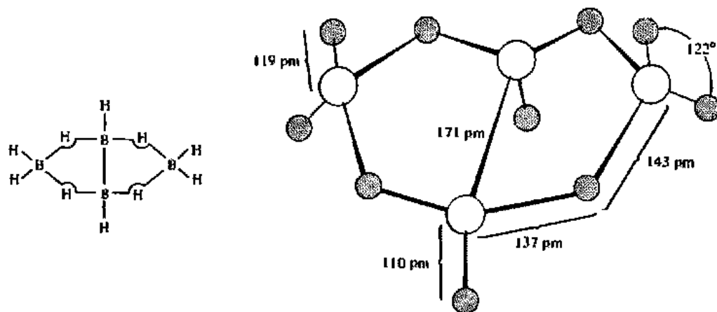
Fig. 16.43 Bonding and structure of tetraborane, B_4H_{10} . [From Muettterties, E. L. The Chemistry of Boron and Its Compounds ; Wiley: New York, 1967. Reproduced with permission.]
