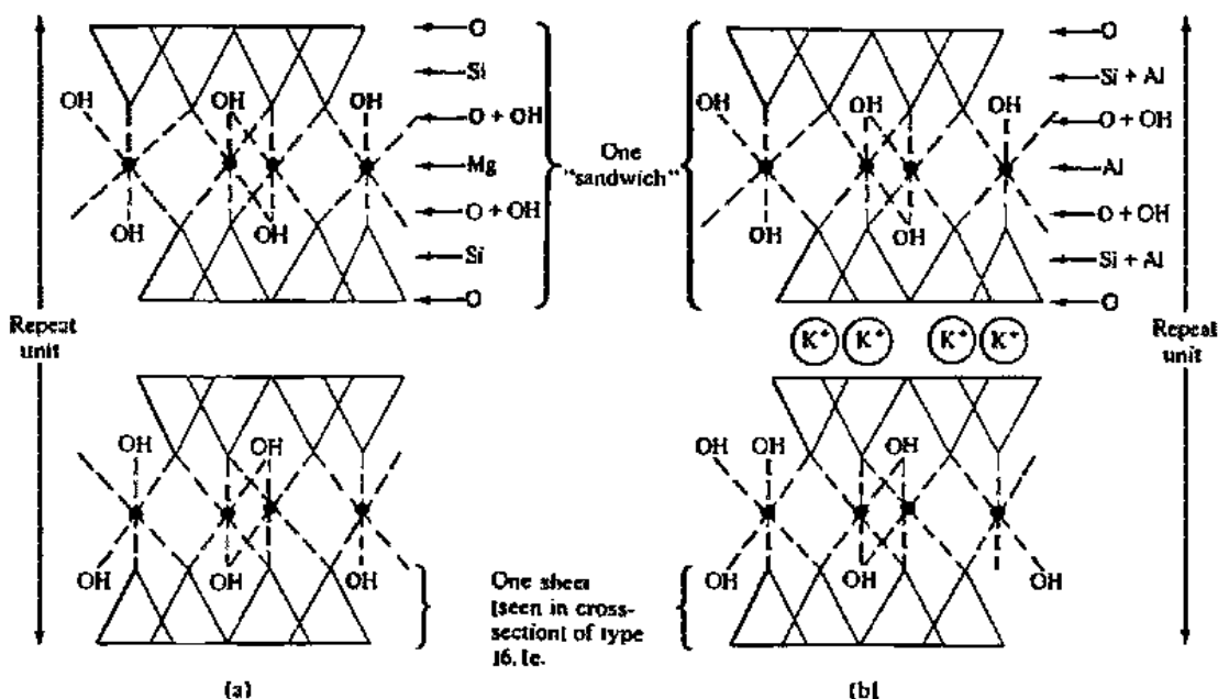
Fig. 16.3 Layered silicate structures: (a) talc, Mg_3(OH)_2(Si_4O_{10}) ; (b) muscovite (a mica) KAl_2(OH)_2Si_3AlO_{10} . [Note: (1) Electroneutrality is maintained by balance of K(I) , Mg(II) , Al(III) , and Si(IV) . (2) The repeating layers in muscovite are bound together by the K^+ cations.] [From Adams, D. M. Inorganic Solids ; Wiley; New York, 1974. Reproduced with permission.]
