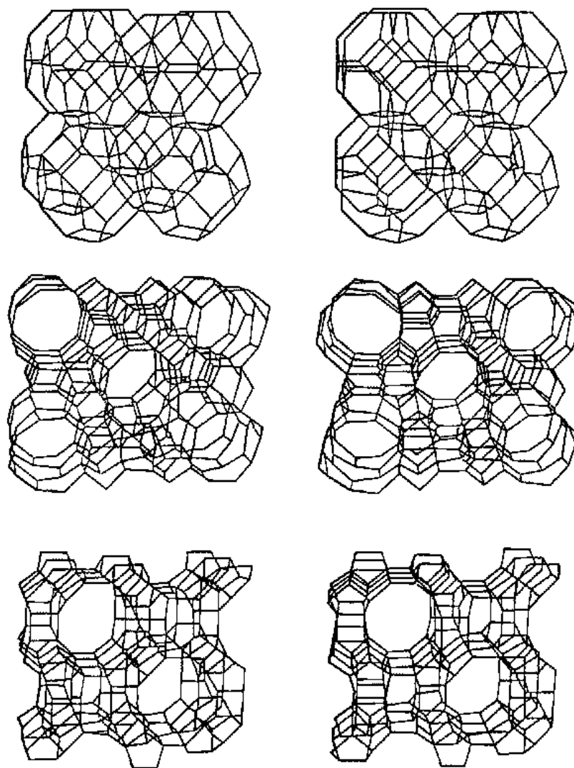
Fig. 16.2 Stereoviews of: (a) sodalite, \text{Na}_4\text{Al}_3\text{Si}_6\text{O}_{24}\cdot 2\text{H}_2\text{O} [ring sizes are 4 and 6 (220 pm)]; (b) ZSM-5, \text{Na}_2\text{Al}_3\text{Si}_9\text{O}_{192}\cdot 16\text{H}_2\text{O} [ring sizes are 4, 5, 6, 7, 8, 10 (580 pm)]; (c) mordenite, \text{Na}_8\text{Al}_8\text{Si}_{40}\text{O}_{96}\cdot 24\text{H}_2\text{O} [ring sizes are 4, 5, 6, 8, 12 (760 pm)]. See also Fig. 1.3. Lines represent oxygen bridges; intersections of lines show positions of the aluminum and silicon atoms. Note increasing size of pore aperture (largest diameter given in parentheses). [From Meier, W. M.; Olson, D. H. Atlas of Zeolite Structure Types , 2nd ed.; Butterworths: London, 1987. Reproduced with permission.]
