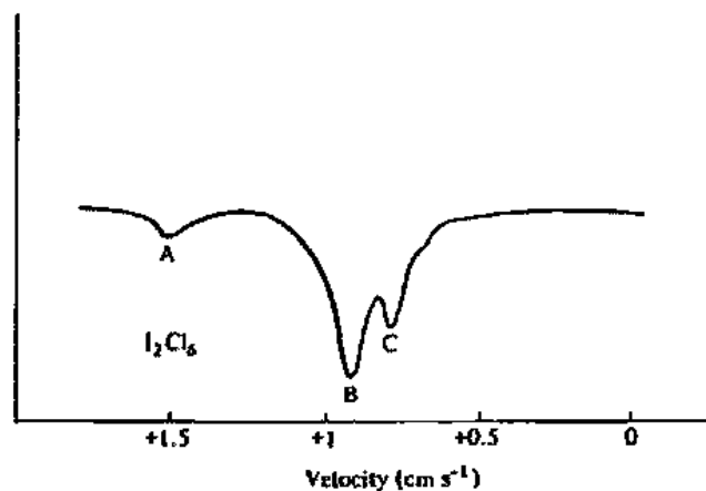
Fig. 6.27 Partial ^{129}\text{I} Mössbauer spectra of \text{I}_2\text{Cl}_6 (top) and \text{I}_2\text{Br}_2\text{Cl}_4 (bottom). Note splitting of peak A in \text{I}_2\text{Cl}_6 into A and A' and B into B' in \text{I}_2\text{Br}_2\text{Cl}_4 . Presumably C' is hidden under a shoulder of B. [From Pasternak, M.; Sonnino, T. J. Chem. Phys. 1968, 48, 1997. Reproduced with permission.]
