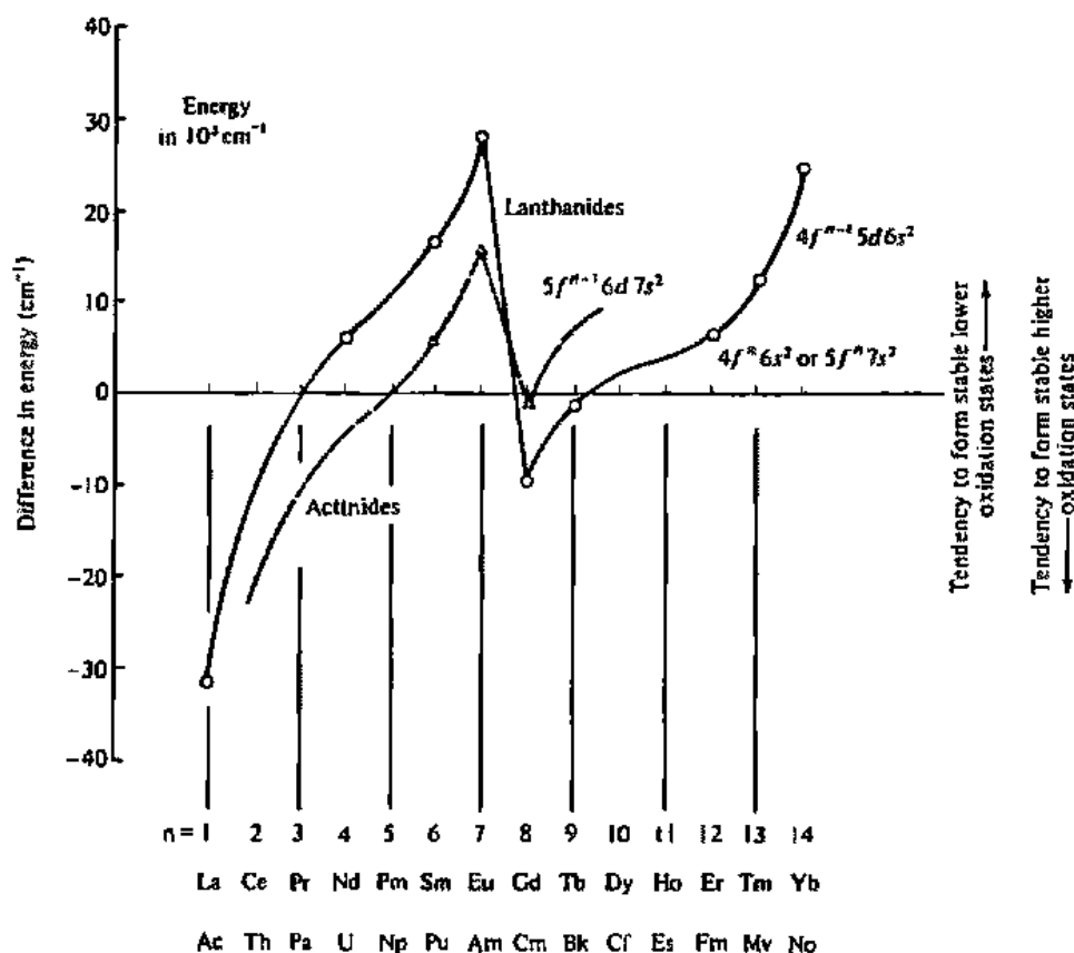
Fig. 14.3 Approximate relative energies of the f^{n-1}d^1s^2 and f^n s^2 electron configurations. [From Fred. M. In Lanthanide/Actinide Chemistry ; Fields, P. R.; Moeller, T., Eds.; Advances in Chemistry 71; American Chemical Society: Washington, DC, 1967. Reproduced with permission.]
