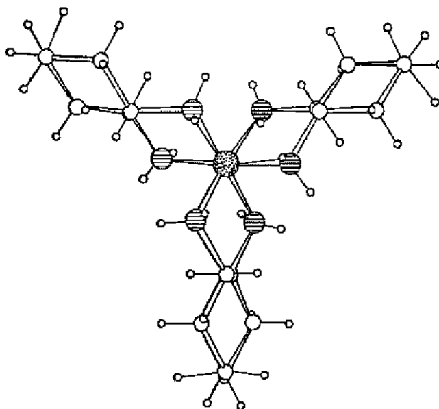
Fig. 12.53 One of two possible enantiomeric solutions to the X-ray crystal structure of the dextrorotatory enantiomer of tris( R,R - trans -1,2-diaminocyclohexane)cobalt(III) cation, (+)_580[\text{Co}(\text{R,R-} \textit{trans}\text{-chxn})_3]^{3+} . See Problem 12.31. [Modified from Saito, Y. Inorganic Molecular Dissymmetry ; Springer-Verlag: Berlin, 1979; p 62. Reproduced with permission.]
