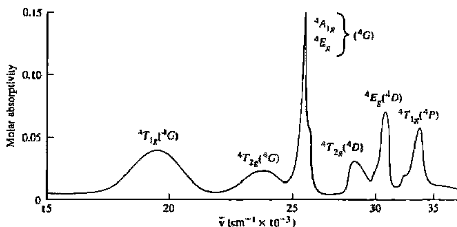
Fig. 11.41 Absorption spectrum for octahedral \text{MnF}_2 . Note the narrow lines. [From Lever, A. B. P. Inorganic Electronic Spectroscopy ; 2nd ed.; Elsevier: New York, 1986; p 45t. Used with permission.]
