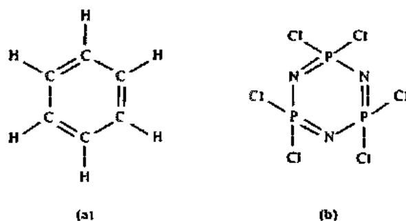
Fig. 5.9 Comparison of bonding in the ring systems of (a) benzene and (b) hexachlororiphoazene.
