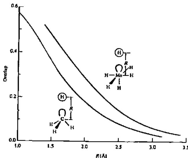
Fig. 15.13 Overlap integrals for the interaction between the a_1 frontier orbital of [\text{MnH}_3]^- or (\text{CH}_3)^- and a 1s orbital on H at a distance R from the Mn or C. [From Hoffmann, R. Angew. Chem. Int. Ed. Engl. 1982, 21, 711-724. Reproduced with permission.]
