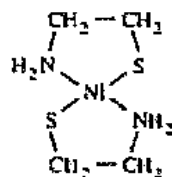
5. trans -isomer
