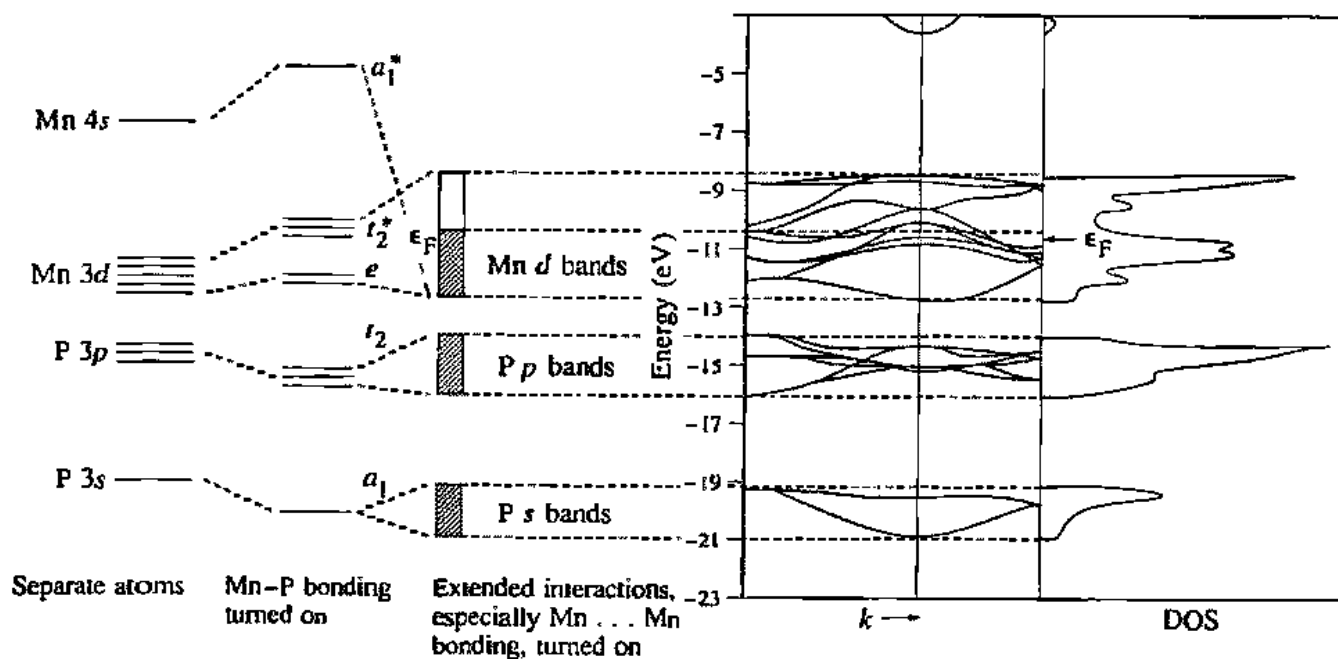
Fig. 7.29 Left: Energy levels of separated Mn and P atoms, Mn-P MO's from adjacent atoms, and extended bonding. Right: Band structure of a single [\text{Mn}_2\text{P}_2]_z^{2-} layer. [Modified from Hoffmann, R.; Zheng, C. J. Phys. Chem. 1985, 89, 4175-4181. Reproduced with permission.]
