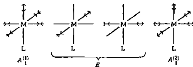
Fig. 11.31 Vibrational stretching modes and their symmetries for M(\text{CO})_3\text{L} complexes.
