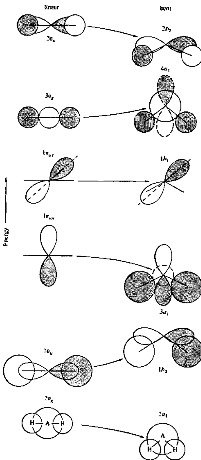
Fig. 6.16 Molecular orbital pictures and qualitative energies of linear and bent AH_2 molecules. Open and shaded areas represent differences in sign (+ or -) of the wave functions. Changes in shape which increase in-phase overlap lower the molecular orbital energy. [From Gimarc, B. M. J. Am. Chem. Soc. 1971, 93, 593. Reproduced with permission.]
