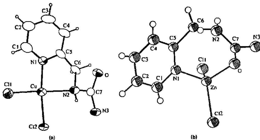
Fig. 12.54 ORTEP drawings of (a) dichloro- N,N' -(2-pyridylmethylurea)copper(II); (b) dichloro- N,O -(2-pyridylmethylurea)zinc(II). [From Maslak, P.; Sczepanski, J. J.; Parvez, M. J. Am. Chem. Soc. 1991, 113, 1062–1063. Reproduced with permission.]
