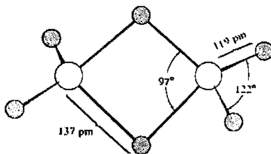
Fig. 16.39 Molecular structure of diborane, B_2H_6 .
