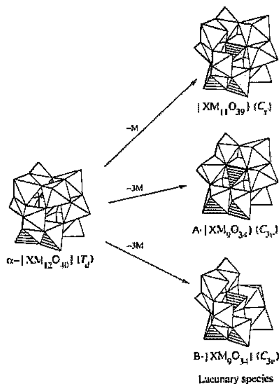
Fig. 16.18 Examples of the polyoxometalate \alpha\text{-[XM}_{12}\text{O}_{40}]^{4-} ion losing both one metal fragment \text{[XM}_{11}\text{O}_{39}] and three metal fragments (isomers A- \text{[XM}_{9}\text{O}_{34}] and B- \text{[XM}_{9}\text{O}_{34}] ). The structures formed (called lacunary structures) have vacant sites which can be filled by other metal fragments. [From Pope, M. T.; Müller, A. Angew. Chem. Int. Ed. Engl. 1991, 30, 34–48. Reproduced with permission.]
