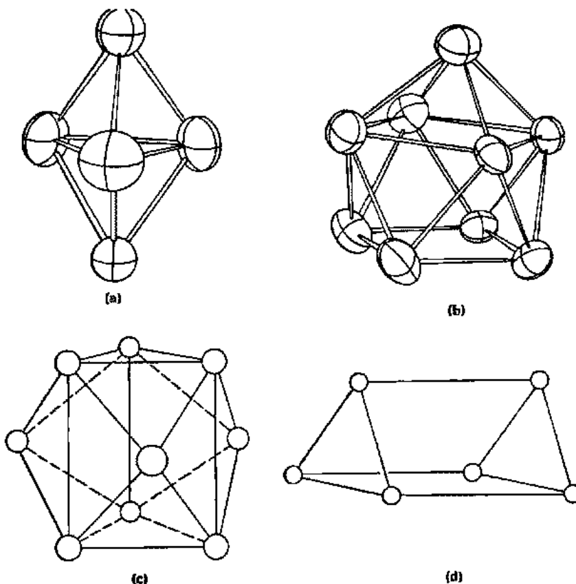
Fig. 16.66 Some representative Zintl ions: (a) \text{Pb}_7^{4-} , (b) \text{Sn}_9^{4-} , (c) \text{Bi}_5^{3+} , (d) \text{Te}_6^{4+} .
