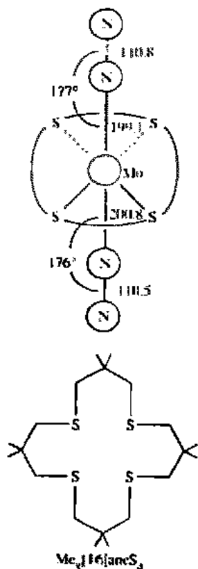
Fig. 15.18 Structure of \text{Mo}(\text{Me}_2[16]\text{aneS}_4)(\text{N}_2)_2 . Bond lengths are in picometers. [From Yoshida, T.; Adachi, T.; Kaminaka, M.; Ueda, T.; Higuchi, T. J. Am. Chem. Soc. 1988, 110, 4872–4873. Used with permission.]
