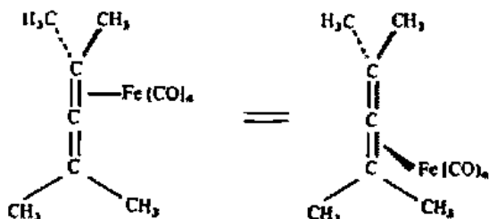
Fig. 15.53 Migration of iron in tetracarbonyltetramethylalleneiron(0).
