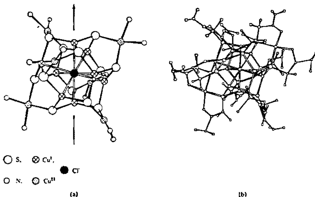
Fig. 19.30 Molecular structure of copper complex of D-penicillamine. The [\text{Cu}_8\text{Cu}_6(\text{penicillaminato})_{12}\text{Cl}] ion: (a) the central cluster of Cu and ligating atoms only; (b) the entire ion with the central cluster oriented as in (a). [From Birker, P. J. M. W. L.; Freeman, H. C. Chem. Commun. 1976, 312. Reproduced with permission.]
