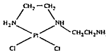
2. didentate chelation
