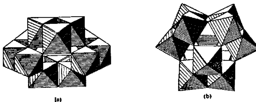
Fig. 16.11 The structures of two apex-shared dodecalungstate isopoly anions; (a) the paratungstate B ion, [H_2W_{12}O_{42}]^{10-} ; (b) the metatungstate ion, [H_2W_{12}O_{40}]^{6-} . [From Lipscomb, W. N. Inorg. Chem. 1965, 4, 132. Reproduced with permission.]
