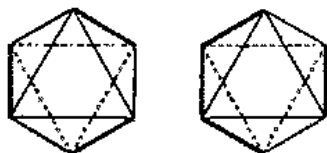
1. delta
