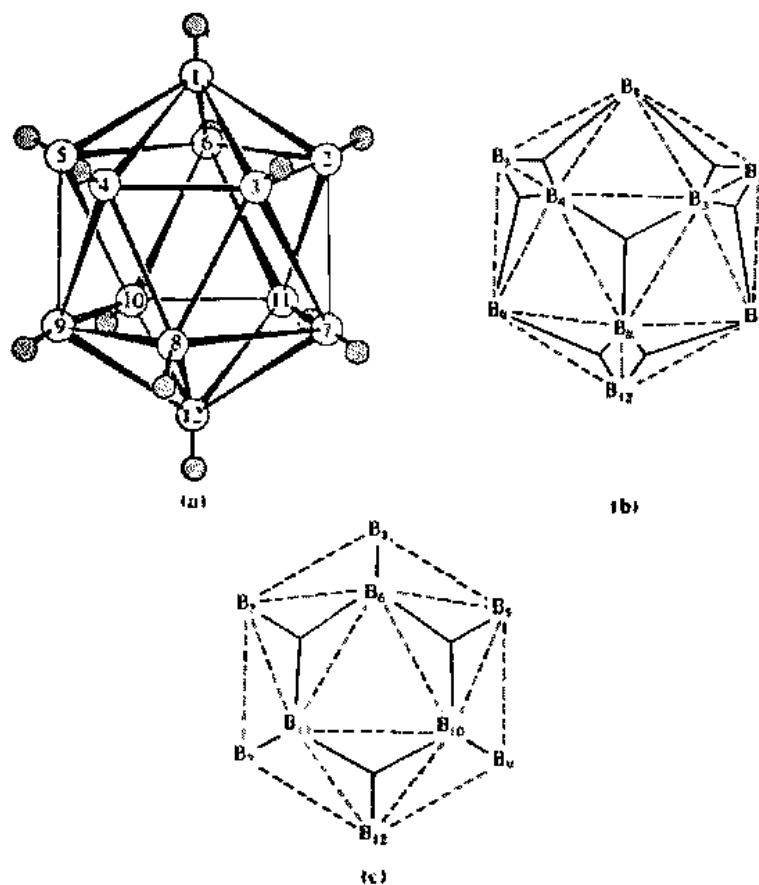
Fig. 16.45 (a) Molecular structure of the [\text{B}_{12}\text{H}_{12}]^{2-} anion; (b), (c) front and back of the [\text{B}_{12}\text{H}_{12}]^{2-} framework showing one of many canonical forms contributing to the resonance hybrid. [(a) From Mueiterties, E. L. The Chemistry of Boron and Its Compounds ; Wiley: New York, 1967; (b) from Jolly, W. L. The Chemistry of the Non-Metals ; Prentice-Hall: Englewood Cliffs, NJ, 1966. Reproduced with permission.]
