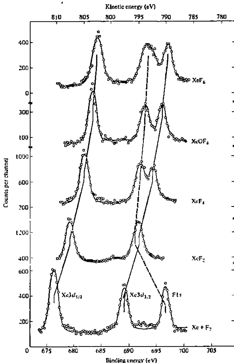
Fig. 17.13 Photoelectron spectra of Xe, \text{F}_2 , \text{XeF}_2 , \text{XeF}_4 , \text{XeOF}_4 , and \text{XeF}_6 . [From Carroll, T. X.; Shaw, R. W., Jr.; Thomas, T. D.; Kindle, C.; Bartlett, N. J. Am. Chem. Soc. 1974, 96, 1989. Reproduced with permission.]
