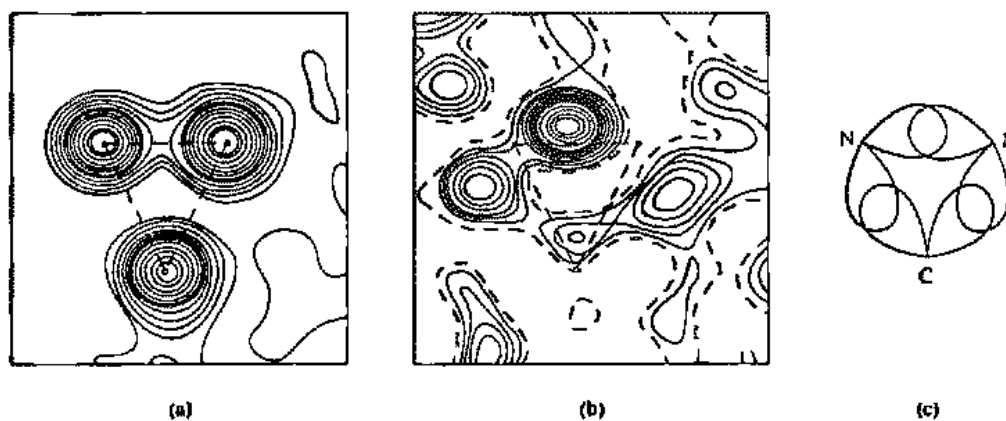
Fig. 6.22 The three-membered C—N—N ring in a diazine molecule: (a) Electron density through the plane of the diazine ring. Contours are at 5 \times 10^{-7} \text{ e pm}^{-3} . (b) Differential electron density map through the plane of the diazine ring showing increases (solid lines) and decreases (broken lines) of electron density upon bond formation. Contours are at 4 \times 10^{-8} \text{ e pm}^{-3} . Note the build-up of electron density outside the C—N—N triangle. The effects can best be seen by superimposing a transparency (as made for overhead projectors, for example) of part (b) over part (a). (c) Interpretation of (a) and (b) in terms of hybrid orbitals. [From Cameron, T. S.; Bakshi, P. K.; Borecka, B.; Liu, M. T. H. J. Am. Chem. Soc. 1992, 114, 1889–1890. Reproduced with permission.]
