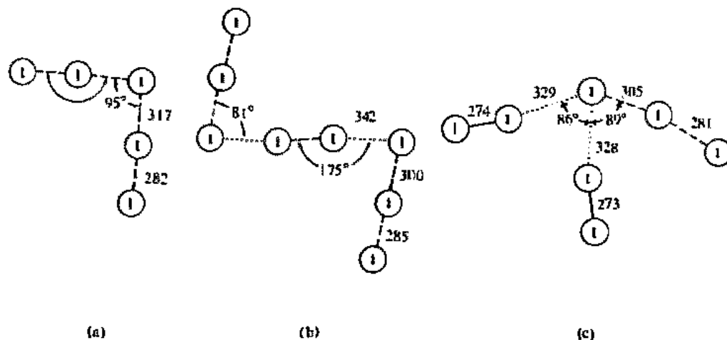
Fig. 17.8 Structures of polyiodide ions: (a) The pentaiodide ion, I_5^- ; (b) the octaiodide ion, I_8^{2-} ; (c) the heptaiodide ion as found in Ph_4P I_7 . Solid lines represent essentially normal covalent bonds, dashed lines represent weakened or partial bonds, and dotted lines represent very long and weak interactions. Distances in pm.
