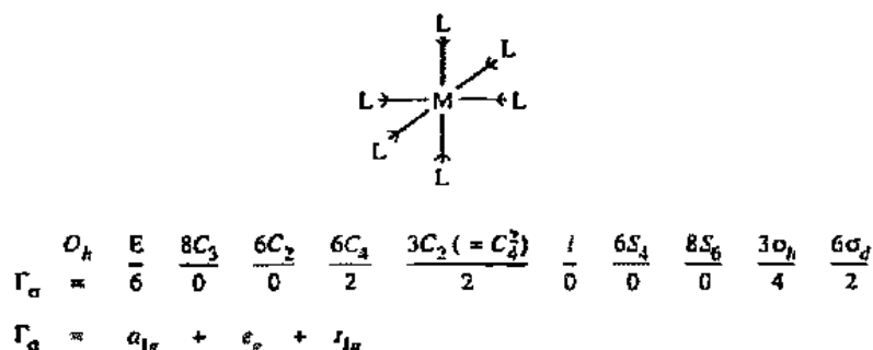
Fig. 11.18 Identification of the symmetries of ligand group orbitals and metal orbitals involved in the \sigma bonds (represented as vectors) of an octahedral ML_6 complex. The characters of the reducible representation, \Gamma_{\sigma} , are derived by counting the number of vectors that remain unmoved under each symmetry operation of the O_h point group. The irreducible components of \Gamma_{\sigma} are obtained by application of Eq. 3.1.
