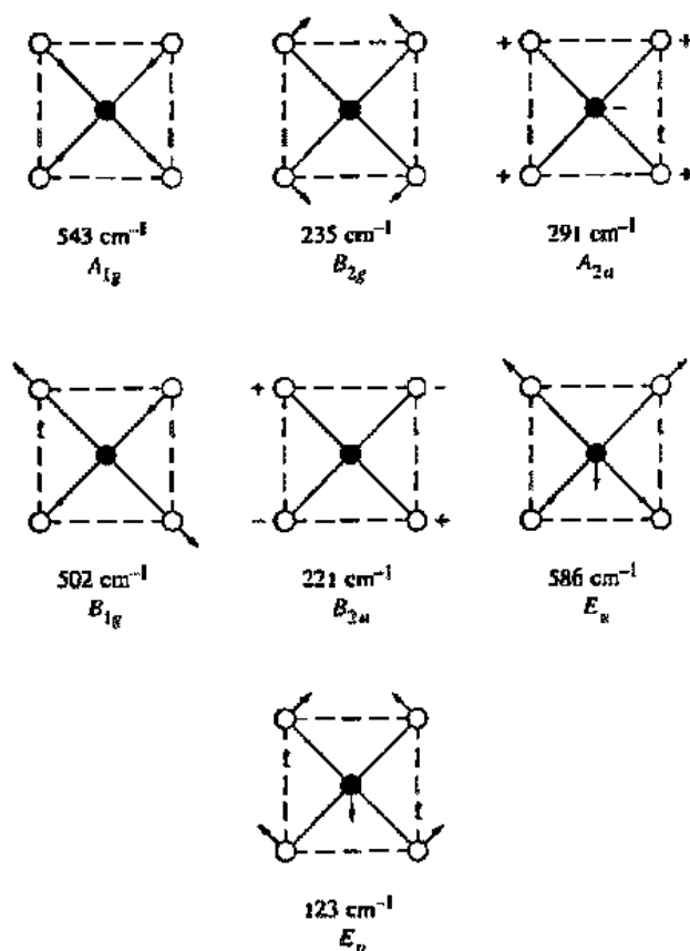
Fig. 3.24 Normal modes of vibration of the \text{XeF}_4 molecule. Note that both E_g modes are doubly degenerate. [Modified from Harris, D. C.; Bertolucci, M. D. Symmetry and Spectroscopy ; Dover: New York, 1989. Used with permission.]
