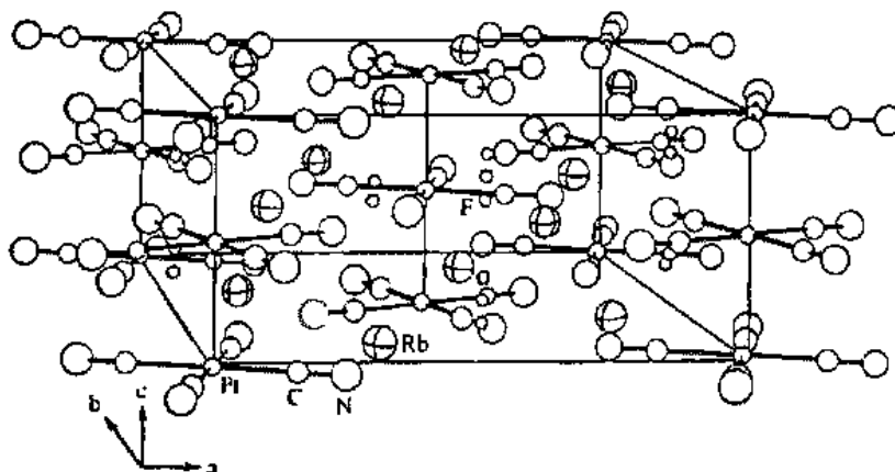
Fig. 16.8 Perspective view of the unit cell of \text{Rb}_2[\text{Pt}(\text{CN})_4](\text{FHF})_{0.50} . One-dimensional chains of staggered [\text{Pt}(\text{CN})_4]^{2-} ions occupy the corners and center of the unit cell. The triad of small circles represents the partially occupied positions of the \text{FHF}^- ions. Note the very short Pt—Pt distance [279.8 pm]. [From Schultz, A. J.; Coffey, C. C.; Lee, G. C.; Williams, J. M. Inorg. Chem. 1977, 6, 2129. Reproduced with permission.]
