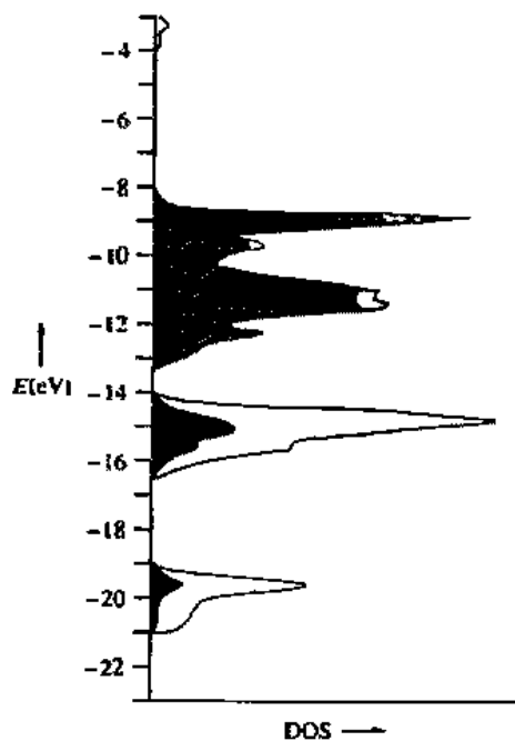
Fig. 7.30 Total DOS of the extended [\text{Mn}_2\text{P}_2]_z^{2-} layer. The relative contributions of the manganese (dark area) and the phosphorus (light area) are indicated. Note that the bonding states at -19 and -15 eV are dominated by the phosphorus, that is, there is more electron density on the phosphorus than on the manganese. [From Hoffmann, R.; Zheng, C. J. Phys. Chem. 1985, 89, 4175-4181. Reproduced with permission.]
