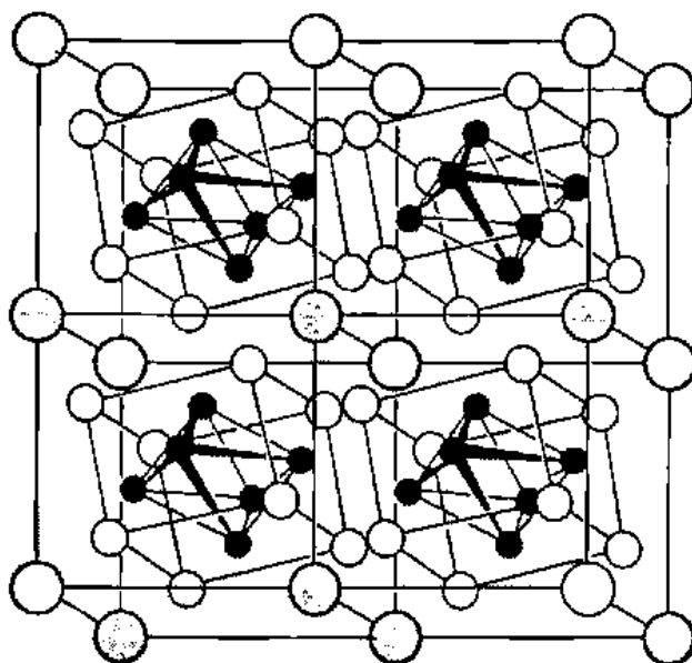
Fig. 16.67 Structure of one of the Chevrel compounds, PbMo_6S_8 . (●) Mo; (○) S; (◐) Pb. [From Colton, F. A. In Reactivity of Metal-Metal Bonds ; Chisholm, M. H., Ed.; ACS Symposium Series 155; American Chemical Society: Washington, DC: 1981. Reproduced with permission.]
