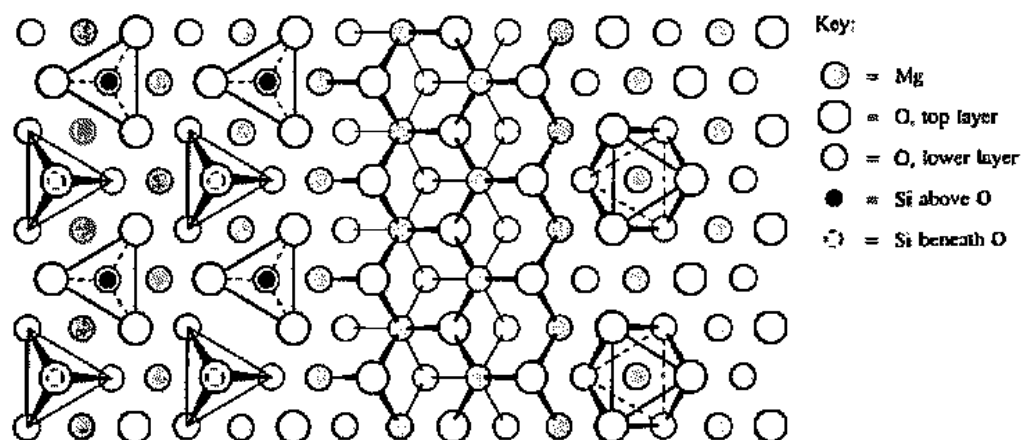
Fig. 7.3 Structure of an olivine, \text{Mg}_2\text{SiO}_4 , portrayed three ways. Left: Discrete \text{SiO}_4^{4-} tetrahedra and \text{Mg}^{2+} ions. Center: Network of Mg—O illustrating the extended structure. The Si atoms have been omitted for clarity. Right: \text{Mg}^{2+} ions in an hcp array of oxide ions. The Si atoms have been omitted. Can you find the tetrahedral holes that they occupy? [Modified from Wells, A. F. Structural Inorganic Chemistry , 5th ed.; Clarendon: Oxford, 1984. Reproduced with permission.]
