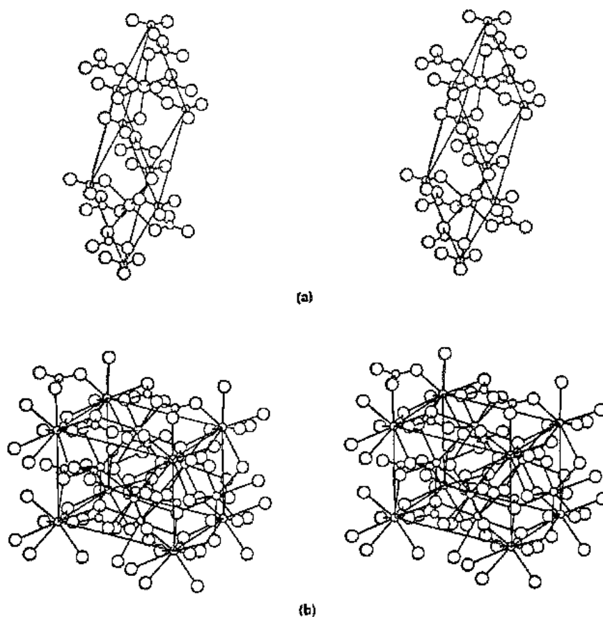
Fig. 4.5 Crystal structures of two forms of calcium carbonate: (a) unit cell of calcite, rhombohedral, space group R\bar{3}c ; (b) unit cell of aragonite, orthorhombic, space group Pcm . Circles in decreasing order of size are oxygen, calcium, and carbon. [From Ladd, M. F. C. Structure and Bonding in Solid State Chemistry ; Wiley: New York, 1979. Reproduced with permission.]
