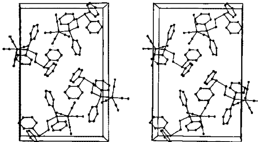
Fig. 3.38 Stereoview of the unit cell of Fe(CO)_4(\eta^1-PPh_2CH_2CH_2PPh_2) . [From Keiser, R. L.; Rheingold, A. L.; Hamerski, J. J.; Castle, C. K. Organometallics 1983, 2, 1635-1639. Reproduced with permission.]
