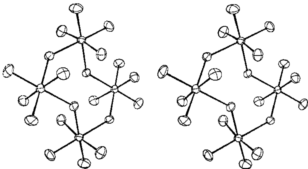
Fig. 7.7 Stereoview of the tetrameric unit of Rh_4F_{20} . The rhodium atoms are at the centers of the octahedra of fluorine atoms. Note bridging fluorine atoms. [From Morrell, B. K.; Zalkin, A.; Tressaud, A.; Bartlett, N. Inorg. Chem. 1973, 12, 2640-2644. Reproduced with permission.]
