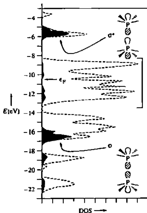
Fig. 7.32 Phosphorus 3p_z orbital contribution (dark area) to the total DOS (dashed line) of the three-dimensional (total) [\text{Mn}_2\text{P}_2]_z^{2-} lattice. The P–P interactions are labeled \sigma and \sigma^* . The square bracket encloses the bands arising principally from the manganese 3d orbitals. [Modified from Hoffmann, R.; Zheng, C. J. Phys. Chem. 1985, 89, 4175–4181. Reproduced with permission.]
