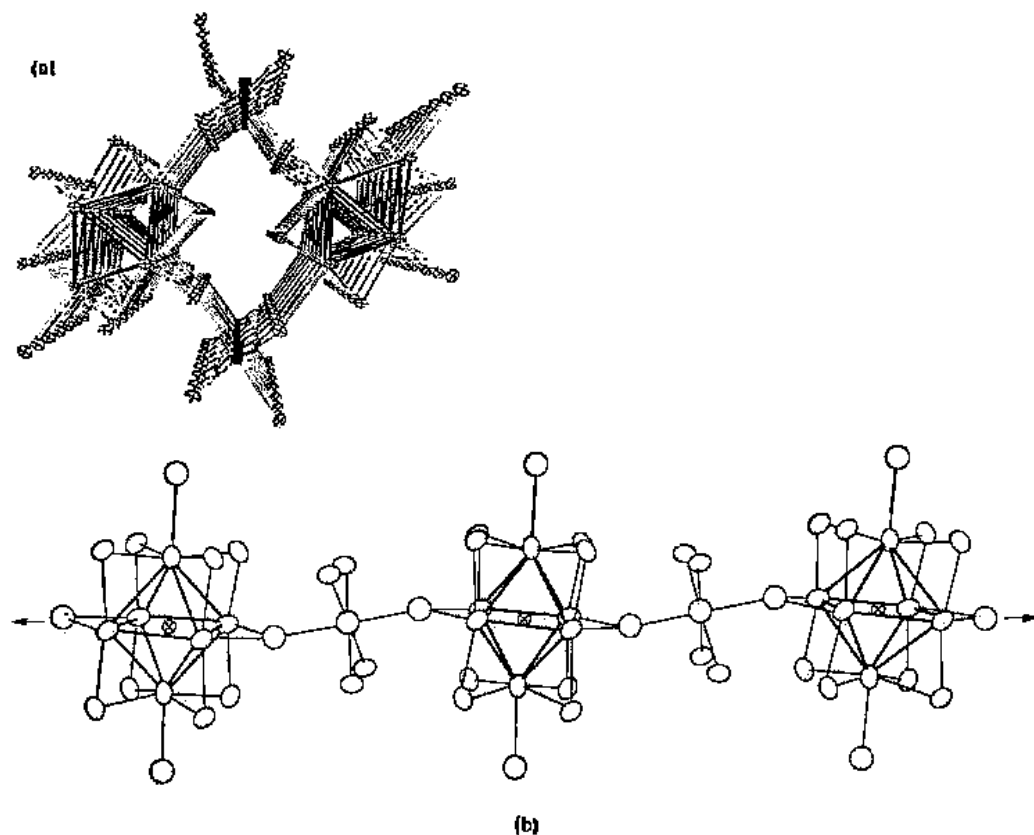
Fig. 16.69 (a) The structure of " Sc_5Cl_{18} " as it was first reported with stacked Sc_6 octahedra (black bonds) and bridging stacked ScCl_6 octahedra (black atoms and white bonds). The poorly scattering nitrogen atoms are not located. (b) The correct structure of Sc_5Cl_{18}N showing Sc_6Cl_{12}N units bridged by ScCl_6 . The interstitial nitrogen atoms lie at the center of the Sc_6 octahedra. Part (a) shows several layers of a pair of these chains. If the nitrogen atoms were shown in (a) they would be stacked in the center of the two columns of stacked black parallelograms, \square . [From Hwu, S.-J.; Dudis, D. S.; Corbett, J. D. Inorg. Chem. 1987, 26, 469–473. Reproduced with permission.]
